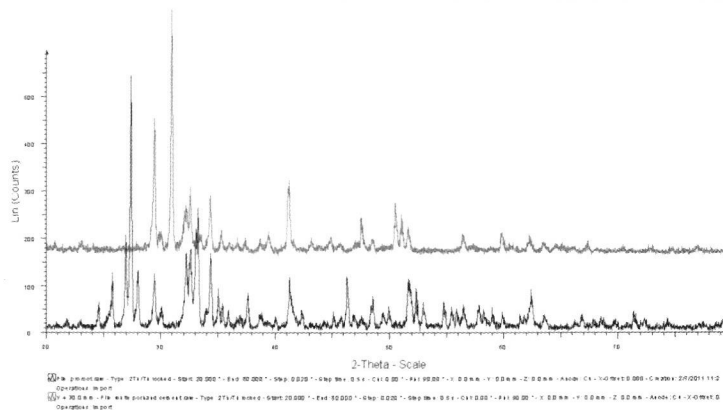
Figure 2. X-ray diffraction analysis results of white Portland cement (upper line) and White ProRoot MTA (lower line) (Unpublished data)
